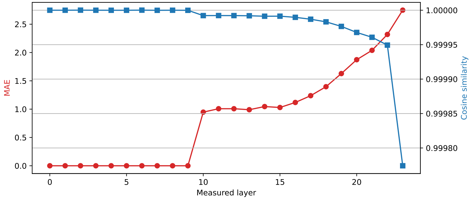
SmolLM2-1.7B-Instruct | Quantized layer 9 | float32 \rightarrow int2
