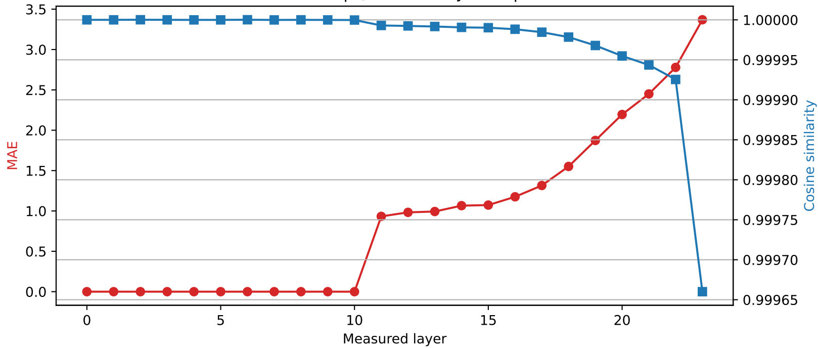
SmolLM2-1.7B-Instruct | Quantized layer 10 | float32 → int2
