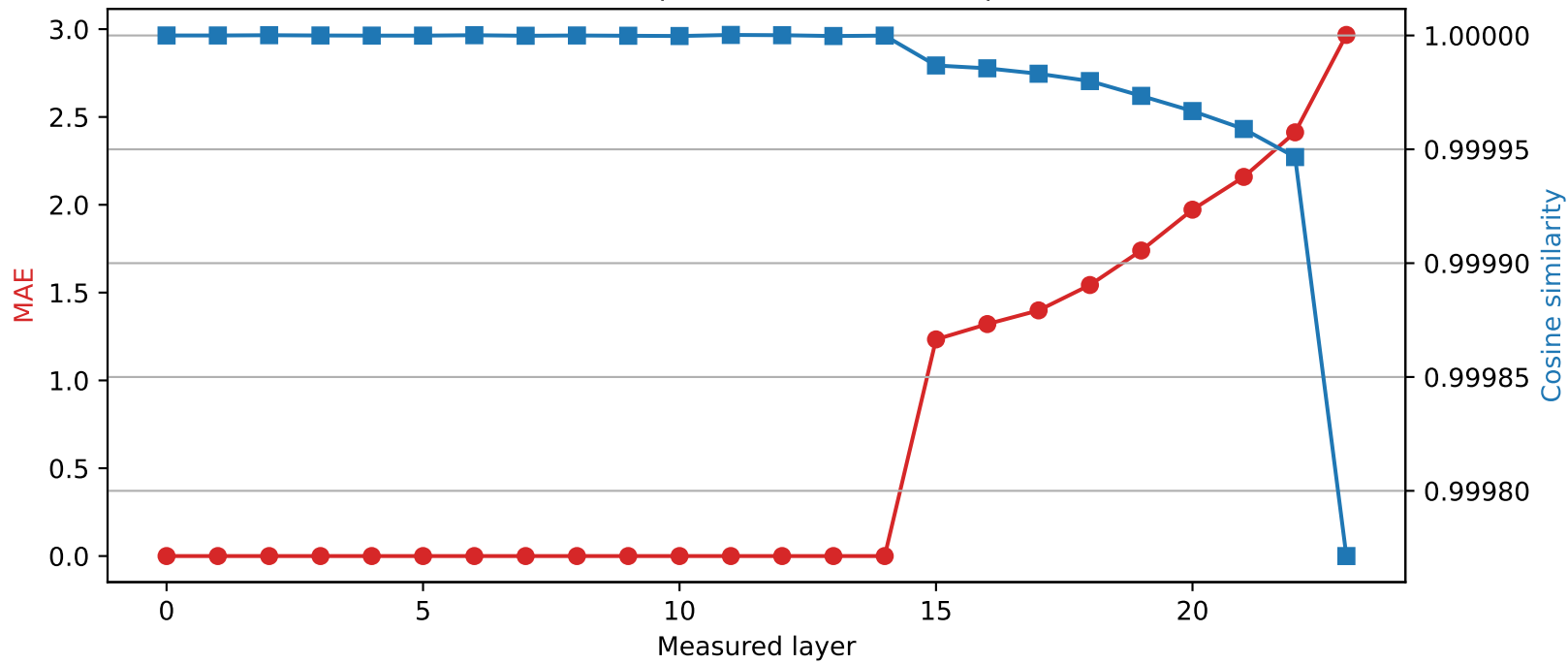
SmolLM2-1.7B-Instruct | Quantized layer 14 | float32 → int2
