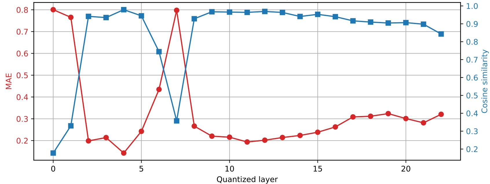
SmolLM2-1.7B-Instruct | Prompt 1 Final RMSNorm output damage | float32 \rightarrow int2
