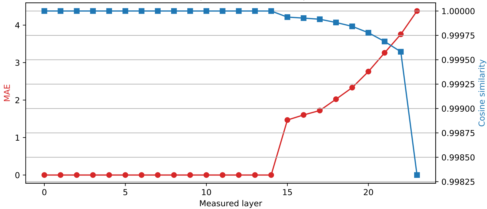
SmolLM2-1.7B-Instruct | Quantized layer 14 | float32 \rightarrow int2
