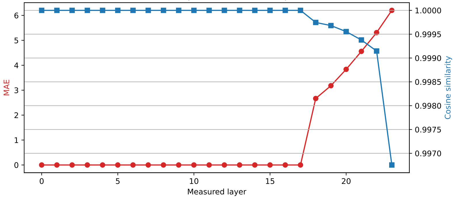
SmolLM2-1.7B-Instruct | Quantized layer 17 | float32 \rightarrow int2
