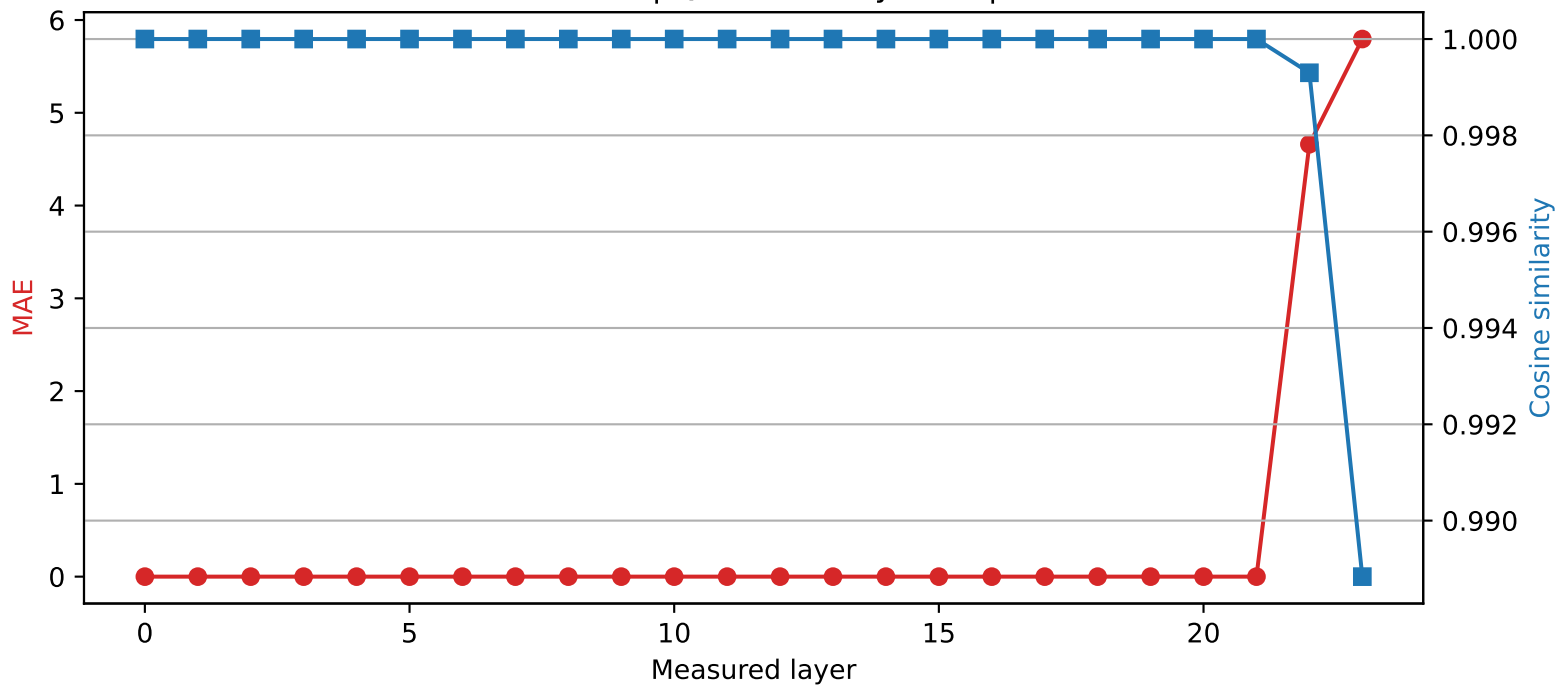
SmolLM2-1.7B-Instruct | Quantized layer 21 | float32 \rightarrow int2
