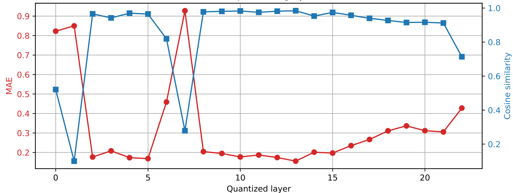
SmolLM2-1.7B-Instruct | Prompt 2 Final RMSNorm output damage | float32 \rightarrow int2
