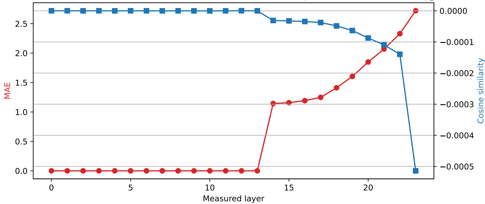
SmolLM2-1.7B-Instruct | Quantized layer 13 | float32 \rightarrow int2
