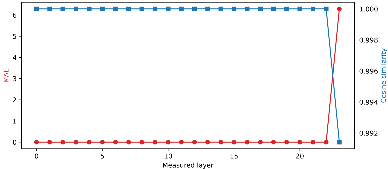
SmolLM2-1.7B-Instruct | Quantized layer 22 | float32 → int2
