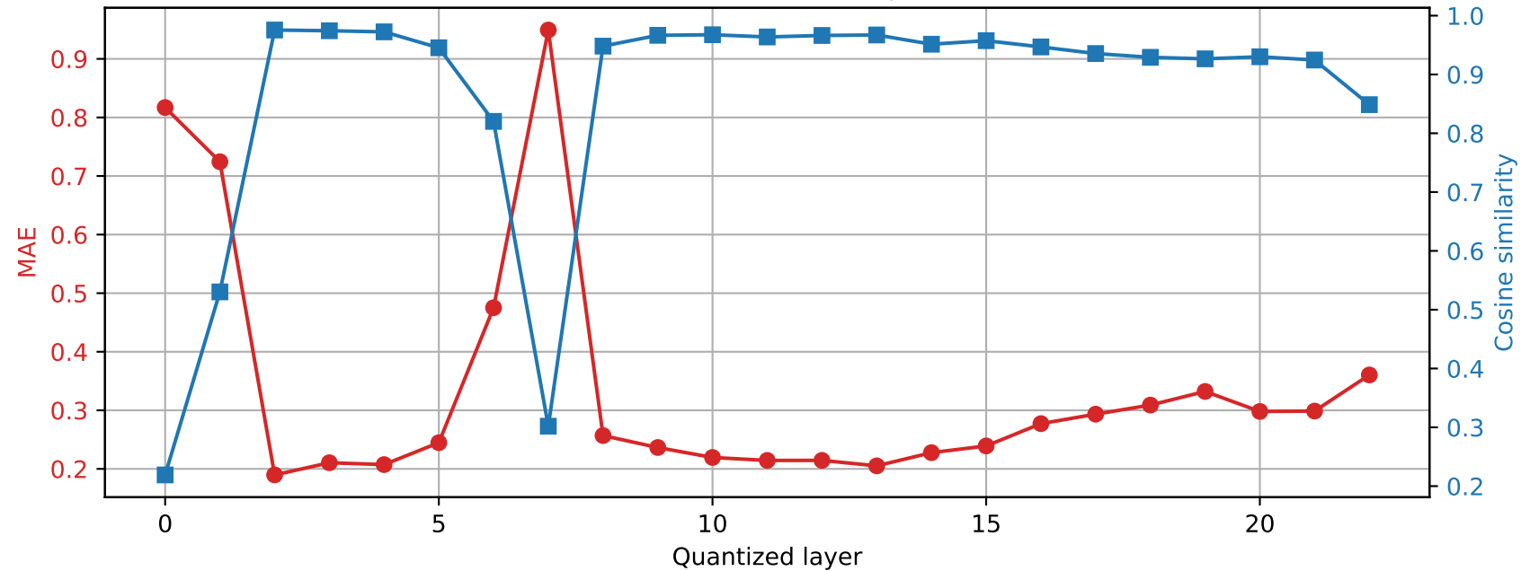
SmolLM2-1.7B-Instruct | Prompt 3 Final RMSNorm output damage | float32 \rightarrow int2
