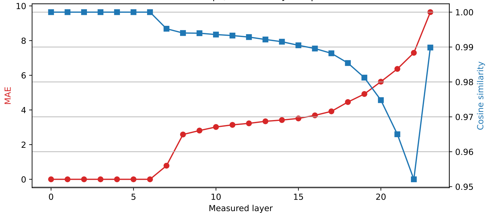
SmolLM2-1.7B-Instruct | Quantized layer 6 | float32 \rightarrow int2
