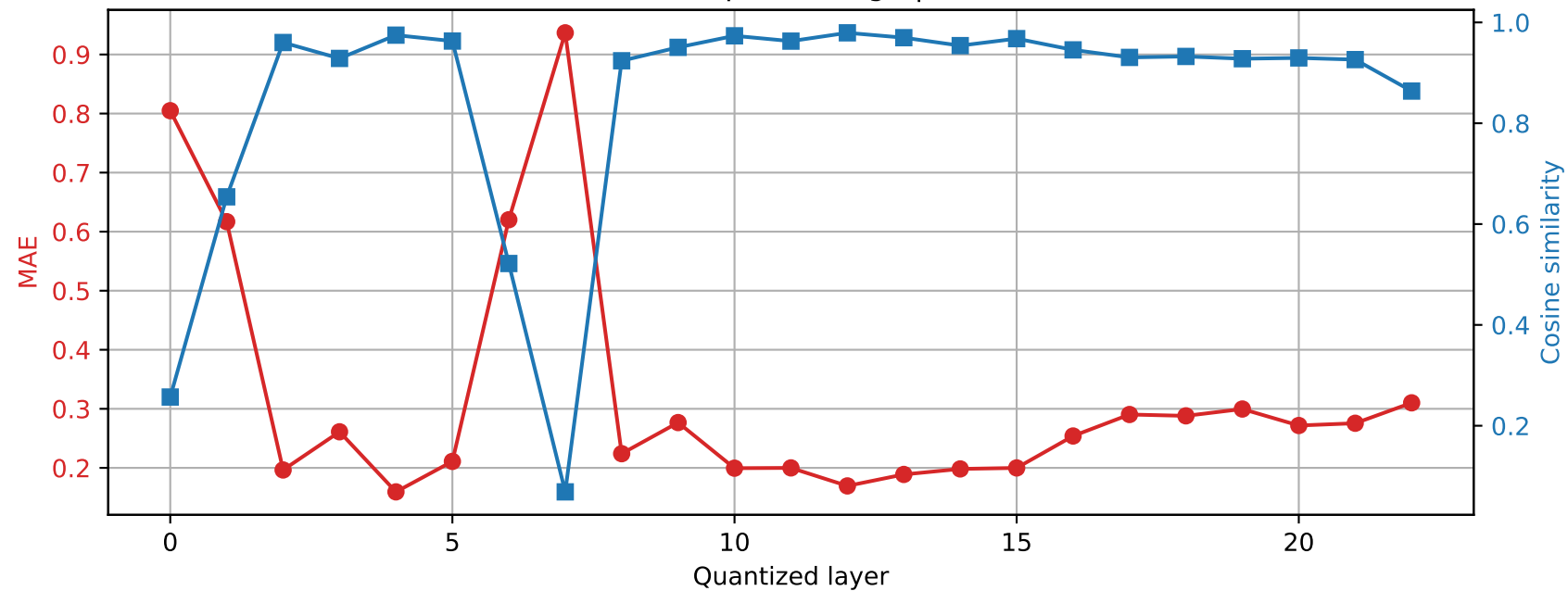
SmolLM2-1.7B-Instruct | Prompt 4 Final RMSNorm output damage | float32 \rightarrow int2
