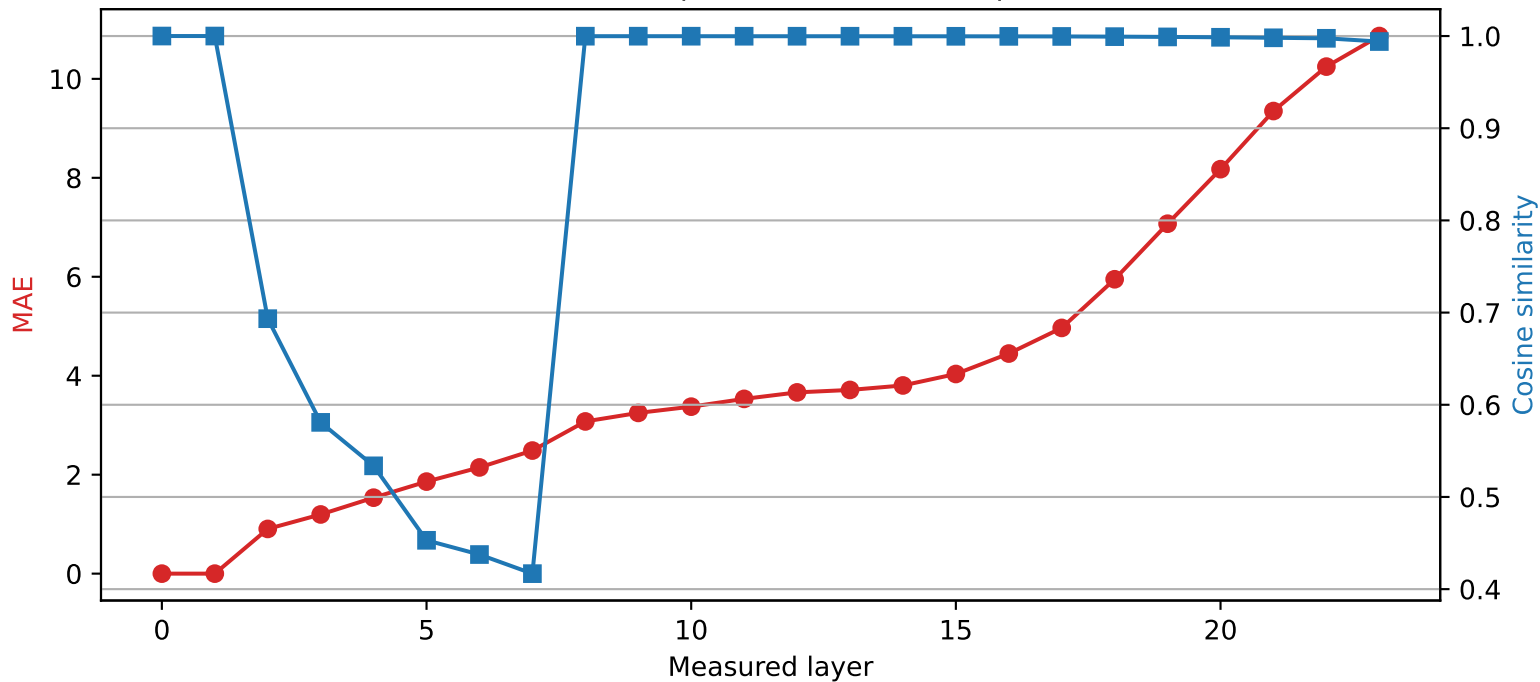
SmolLM2-1.7B-Instruct | Quantized layer 1 | float32 → int2
