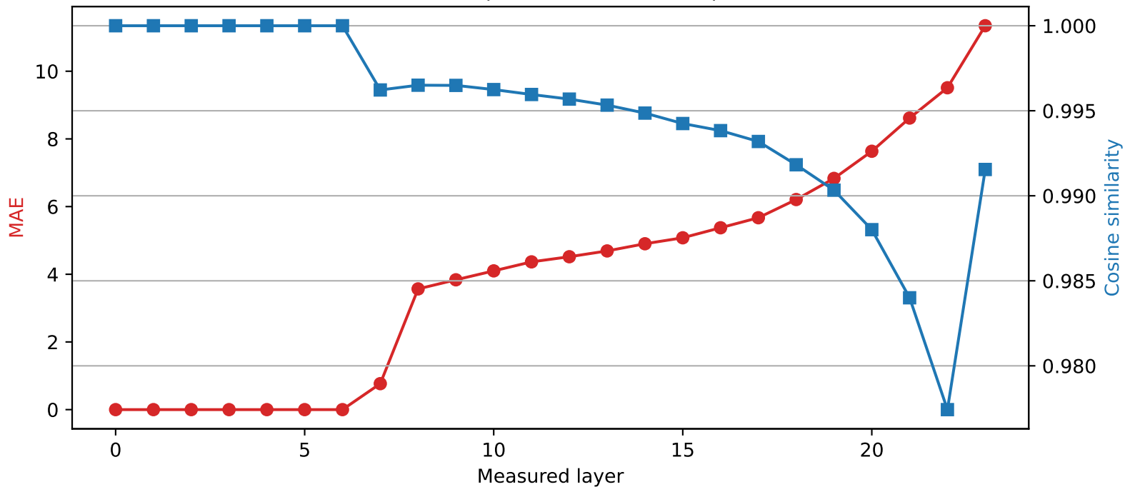
SmolLM2-1.7B-Instruct | Quantized layer 6 | float32 → int2
