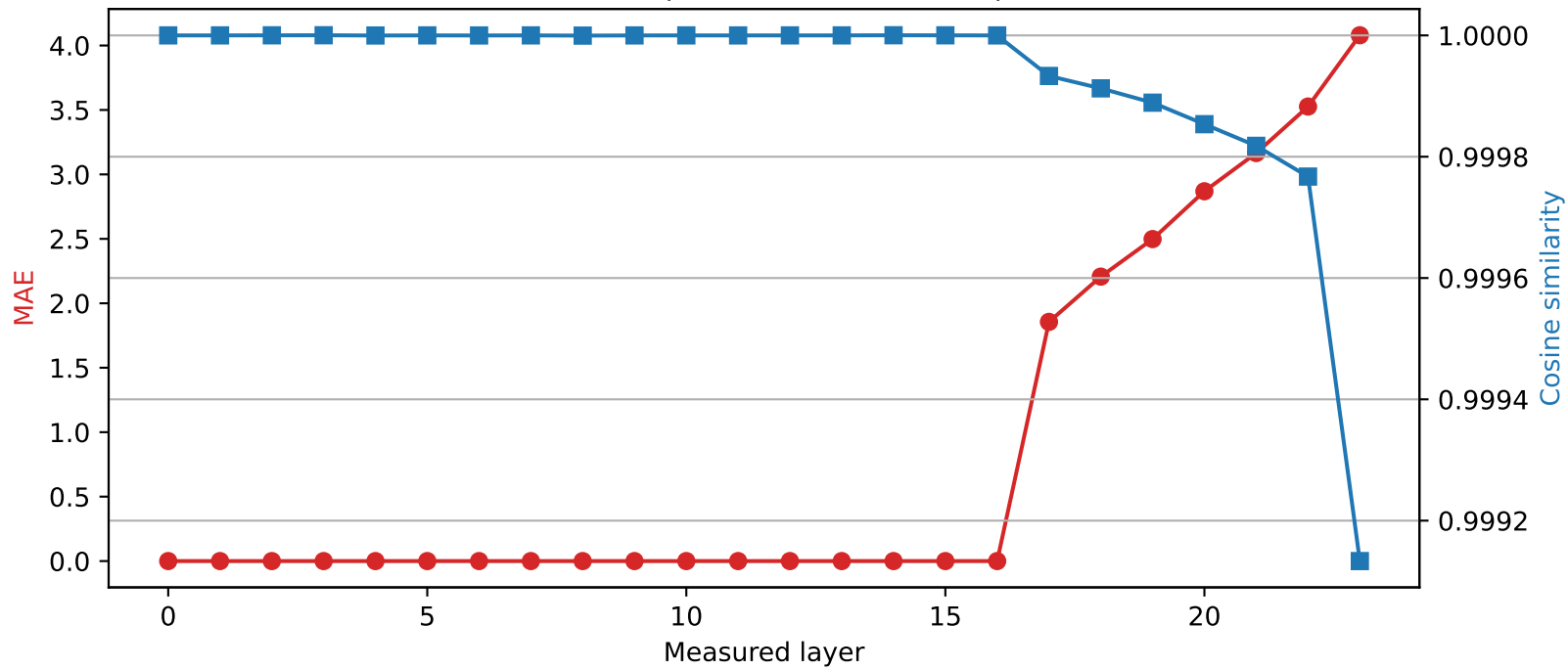
SmolLM2-1.7B-Instruct | Quantized layer 16 | float32 \rightarrow int2
