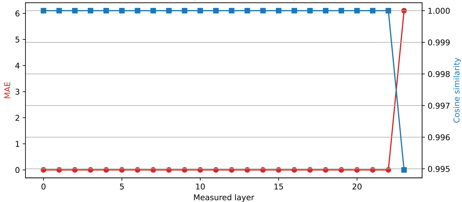
SmolLM2-1.7B-Instruct | Quantized layer 22 | float32 \rightarrow int2
