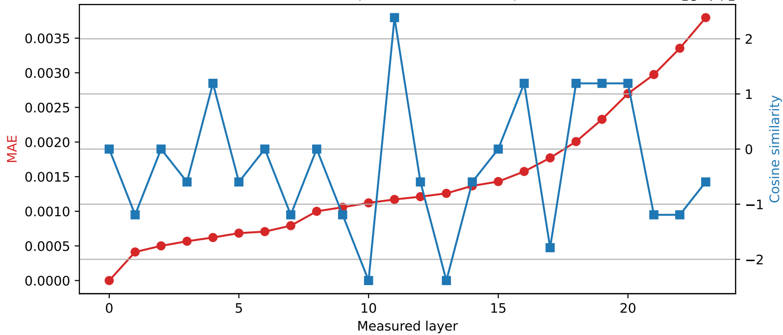
SmolLM2-1.7B-Instruct | Quantized layer 0 | float64 \rightarrow int16
