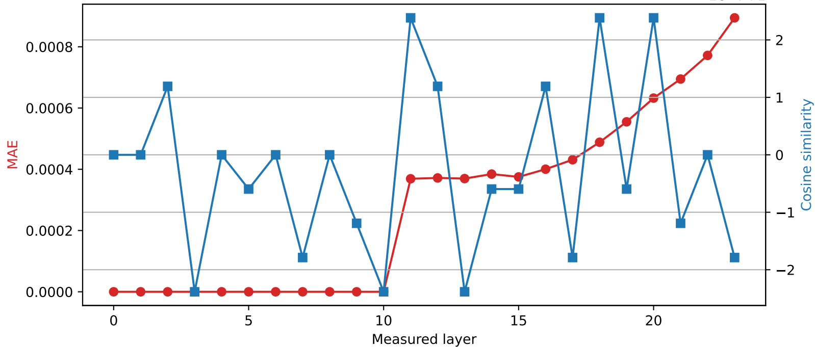
SmolLM2-1.7B-Instruct | Quantized layer 10 | float64 → int16
