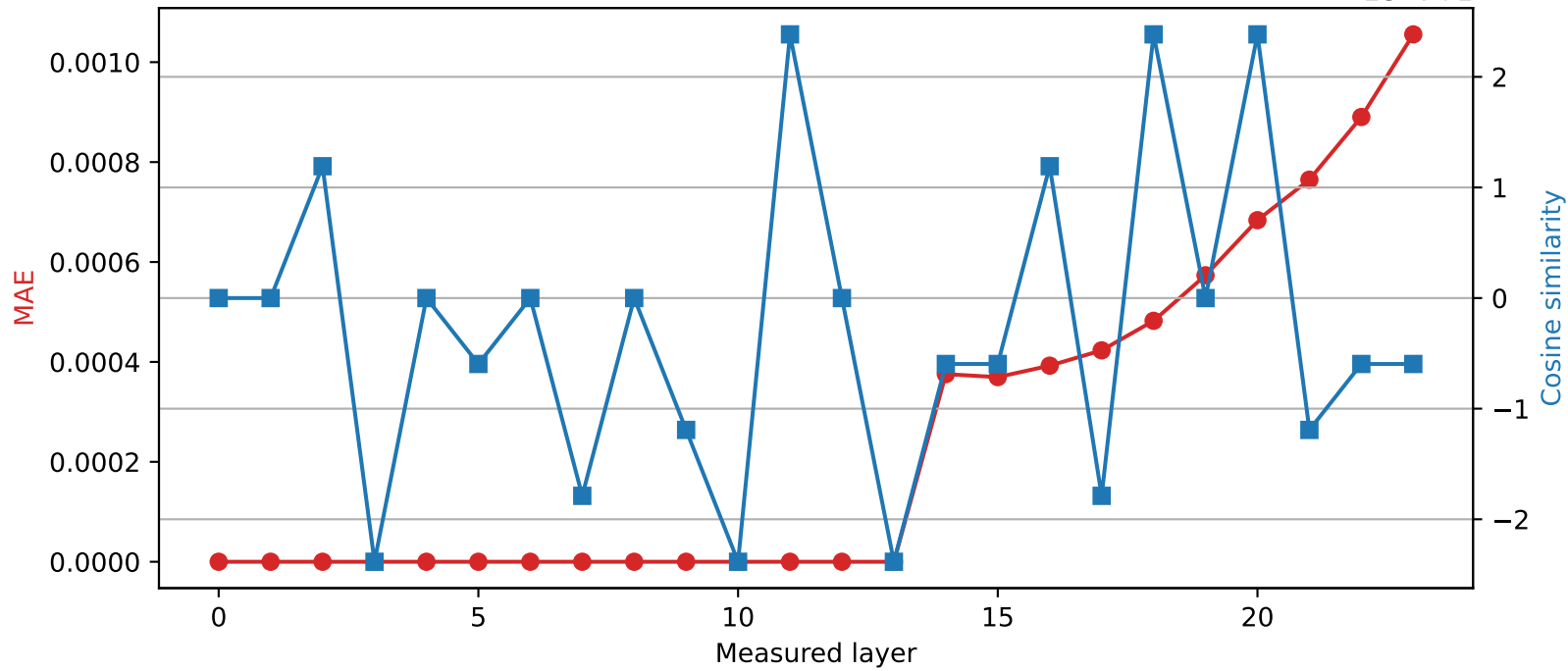
SmolLM2-1.7B-Instruct | Quantized layer 13 | float64 → int16
