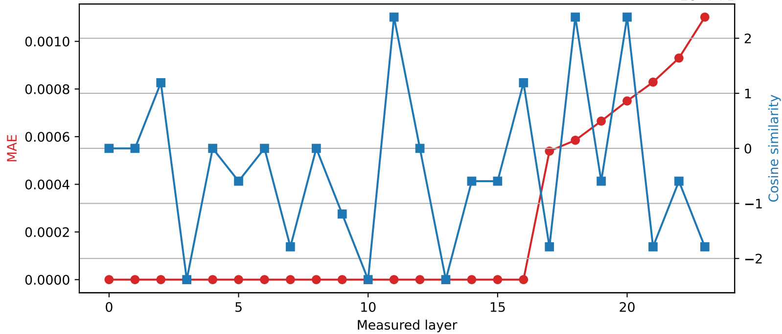
SmolLM2-1.7B-Instruct | Quantized layer 16 | float64 \rightarrow int16
