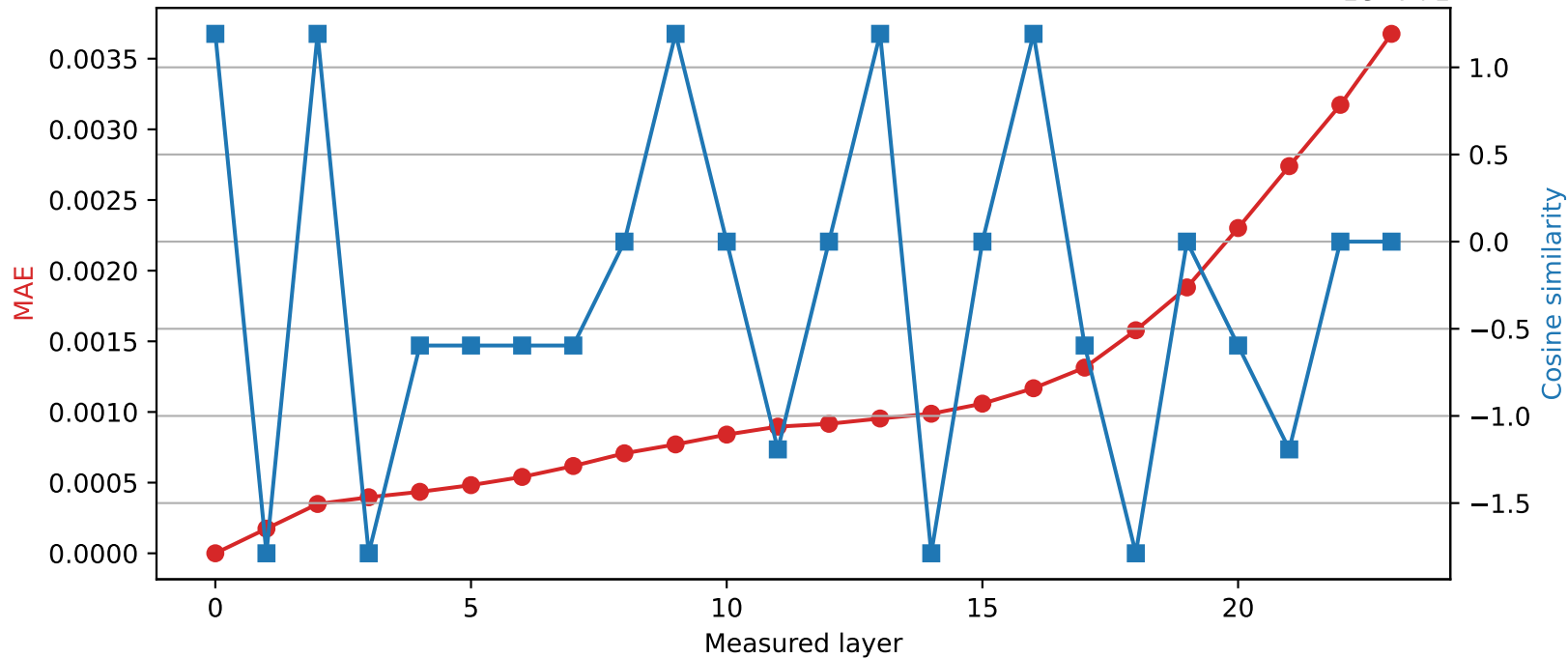
SmolLM2-1.7B-Instruct | Quantized layer 0 | float64 → int16
