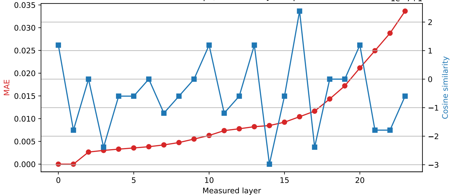
SmolLM2-1.7B-Instruct | Quantized layer 1 | float64 \rightarrow int16
