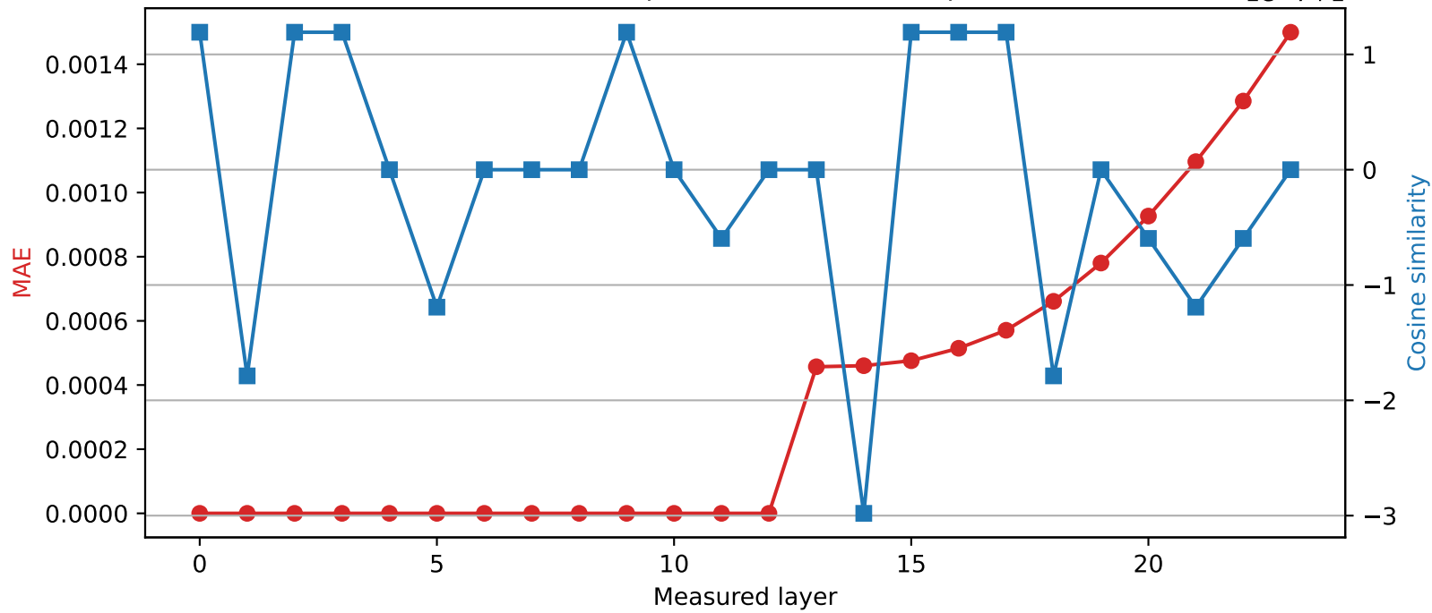
SmolLM2-1.7B-Instruct | Quantized layer 12 | float64 \rightarrow int16
