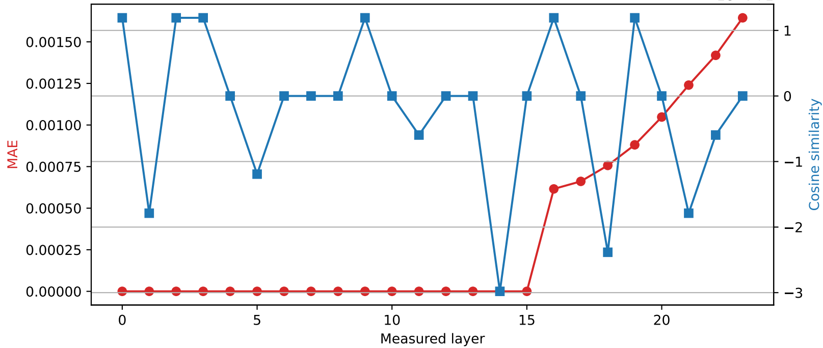
SmolLM2-1.7B-Instruct | Quantized layer 15 | float64 \rightarrow int16
