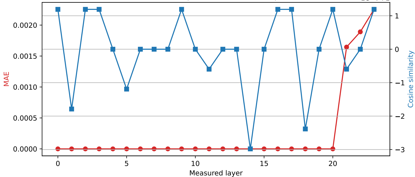
SmolLM2-1.7B-Instruct | Quantized layer 20 | float64 → int16
