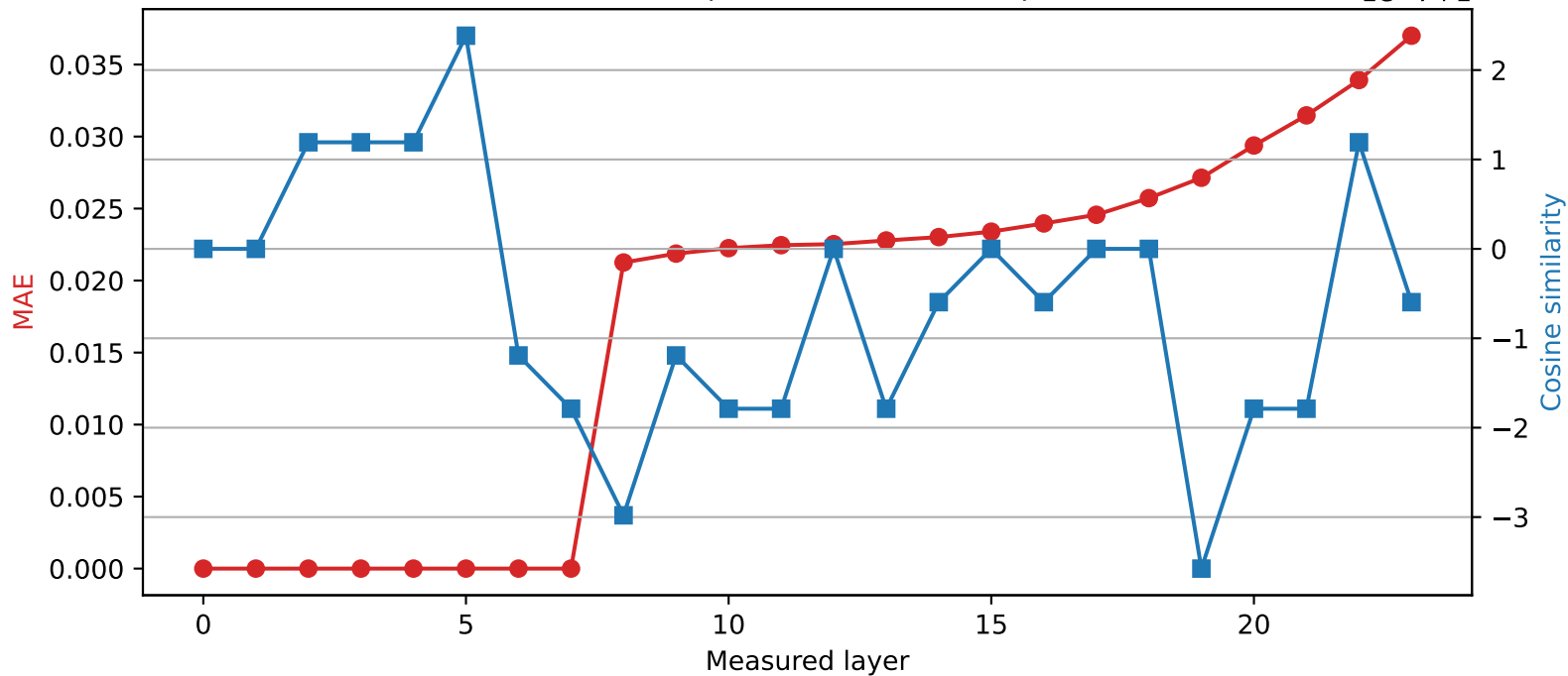
SmolLM2-1.7B-Instruct | Quantized layer 7 | float64 \rightarrow int16
