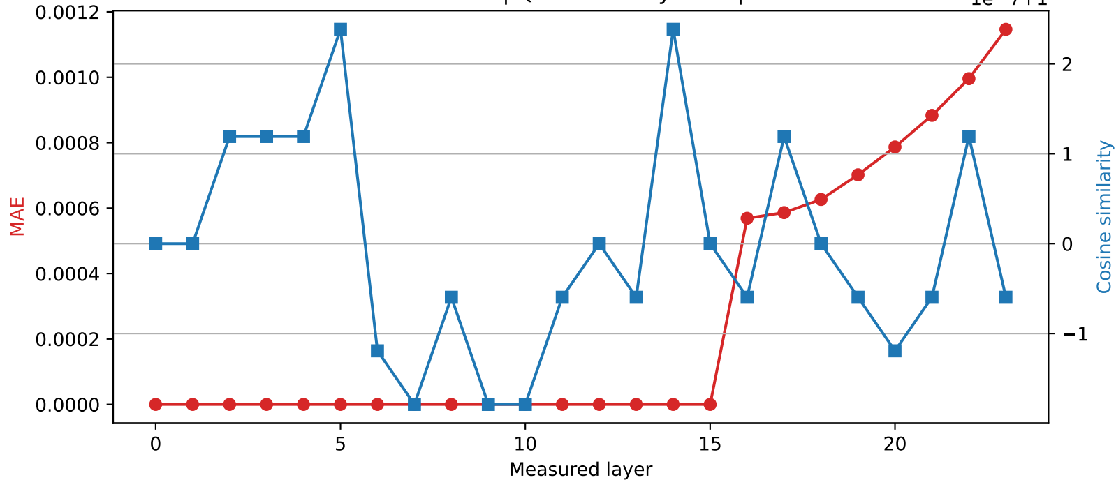
SmolLM2-1.7B-Instruct | Quantized layer 15 | float64 → int16
