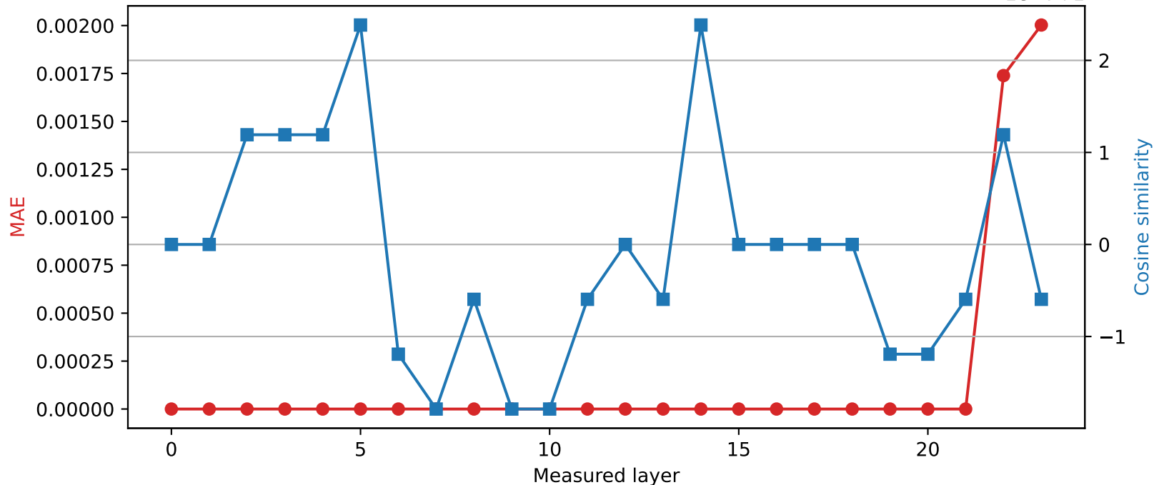
SmolLM2-1.7B-Instruct | Quantized layer 21 | float64 \rightarrow int16
