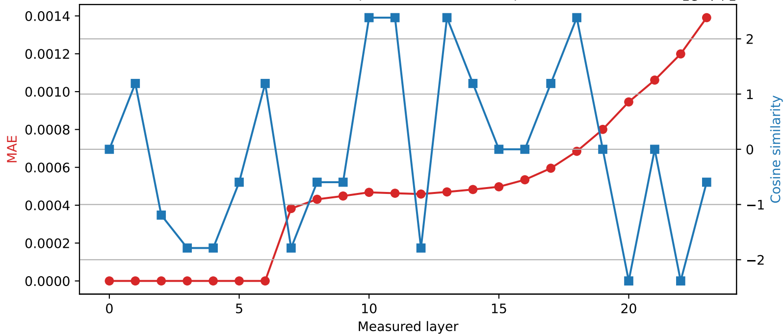
SmolLM2-1.7B-Instruct | Quantized layer 6 | float64 → int16
