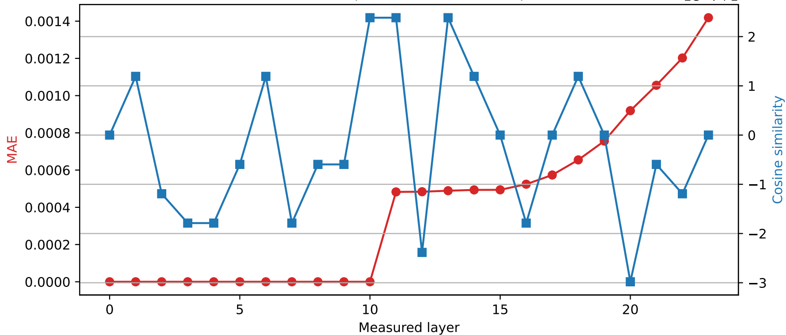
SmolLM2-1.7B-Instruct | Quantized layer 10 | float64 \rightarrow int16
