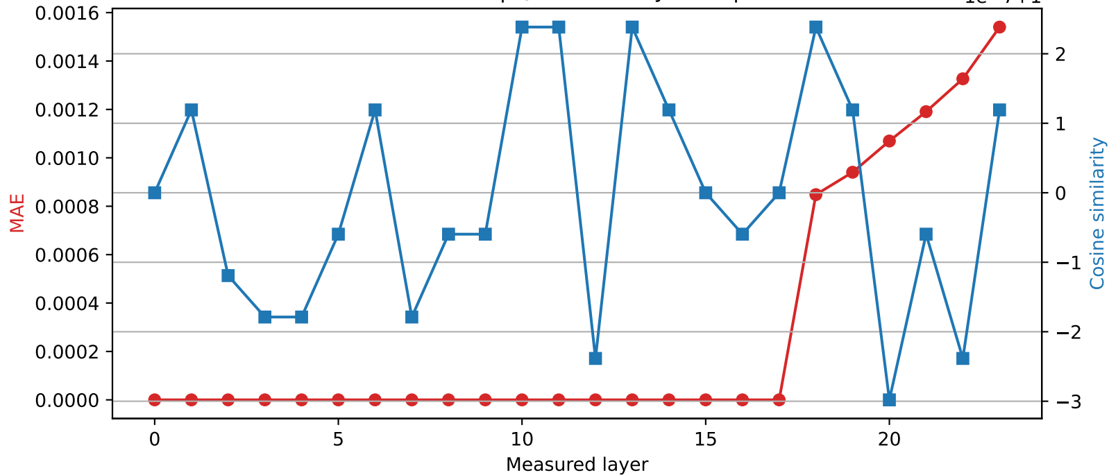
SmolLM2-1.7B-Instruct | Quantized layer 17 | float64 \rightarrow int16
