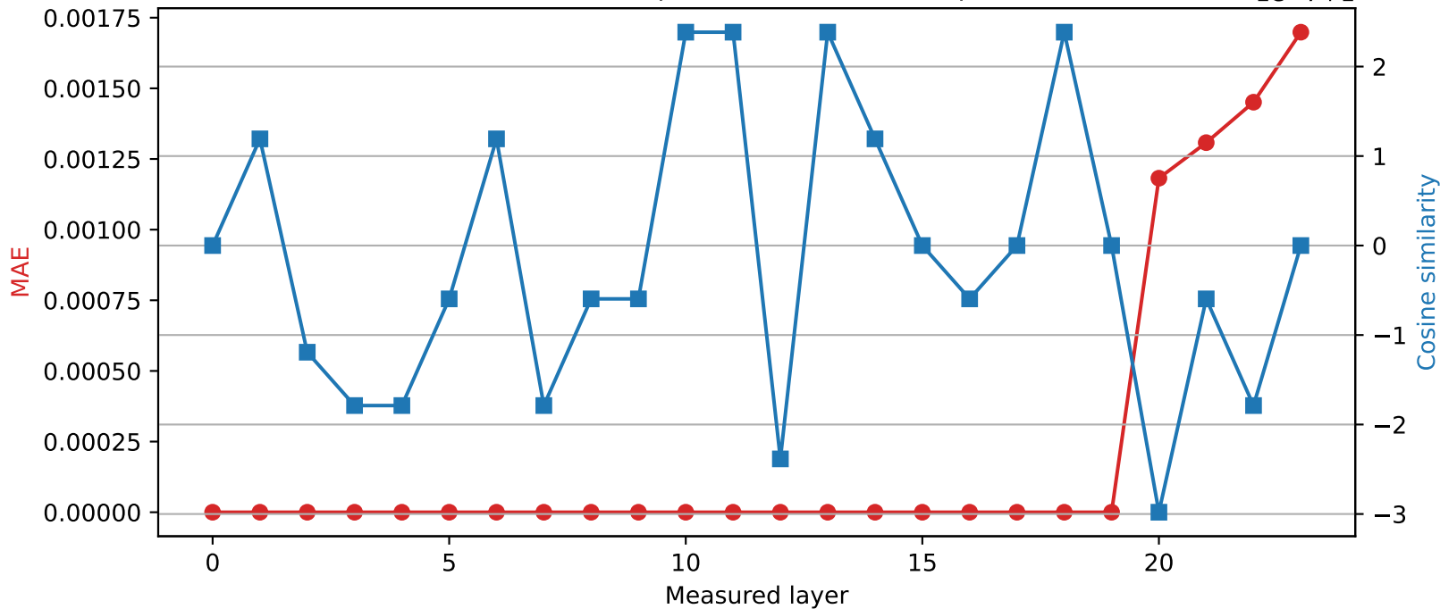
SmolLM2-1.7B-Instruct | Quantized layer 19 | float64 \rightarrow int16
