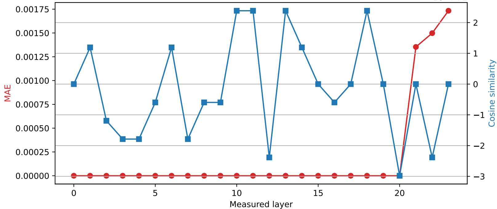
SmolLM2-1.7B-Instruct | Quantized layer 20 | float64 \rightarrow int16
