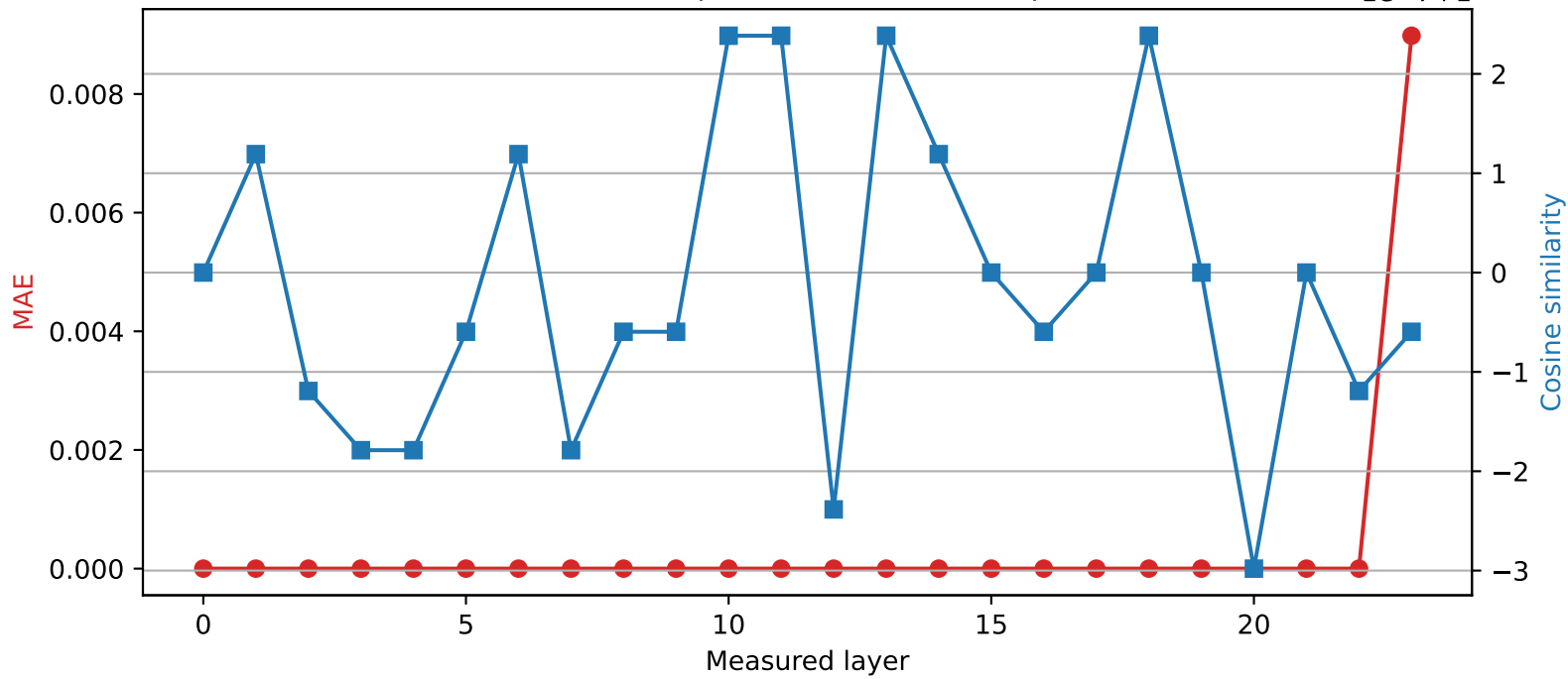
SmolLM2-1.7B-Instruct | Quantized layer 22 | float64 → int16
