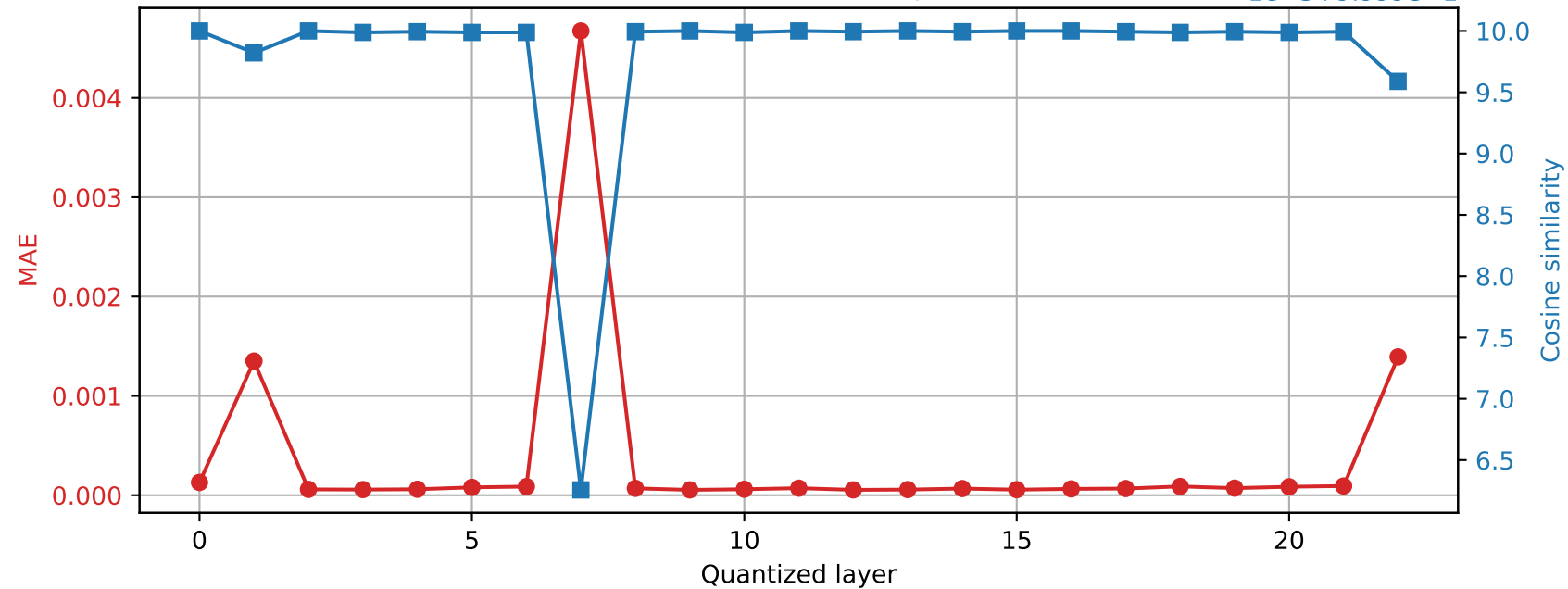
SmolLM2-1.7B-Instruct | Prompt 4 Final RMSNorm output damage | float64 → int16
