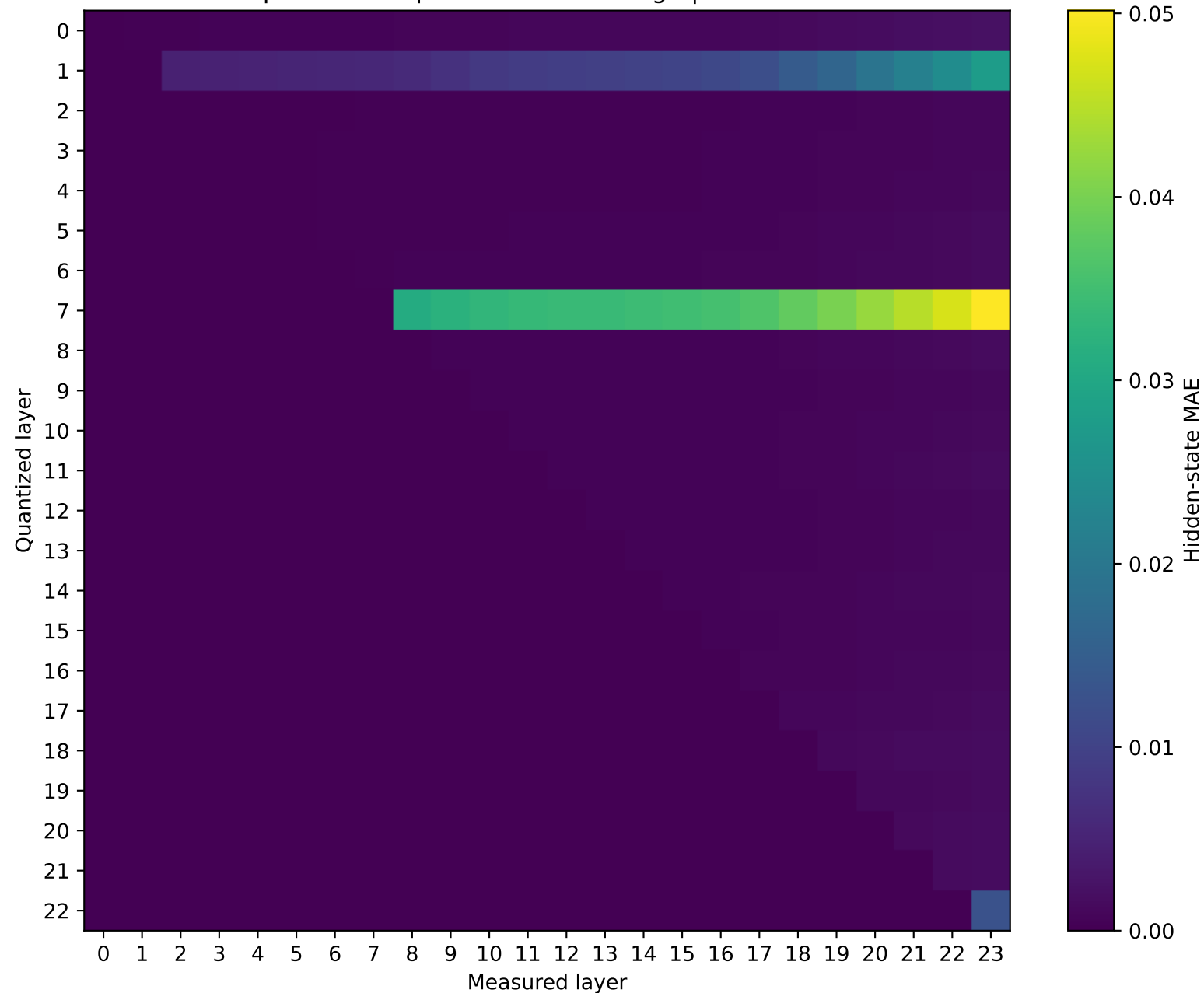
SmolLM2-1.7B-Instruct Prompt 4: MAE representation damage | float64 → int16
