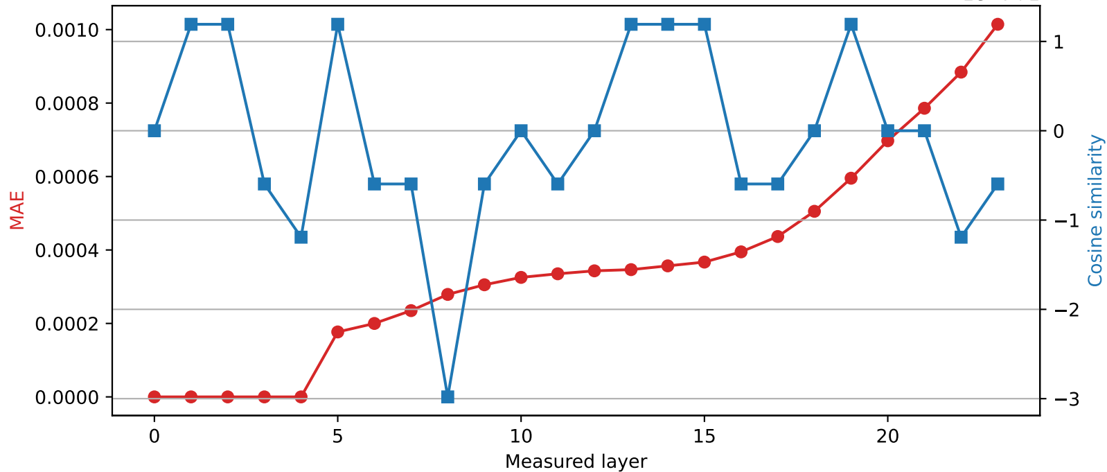
SmolLM2-1.7B-Instruct | Quantized layer 4 | float64 → int16
