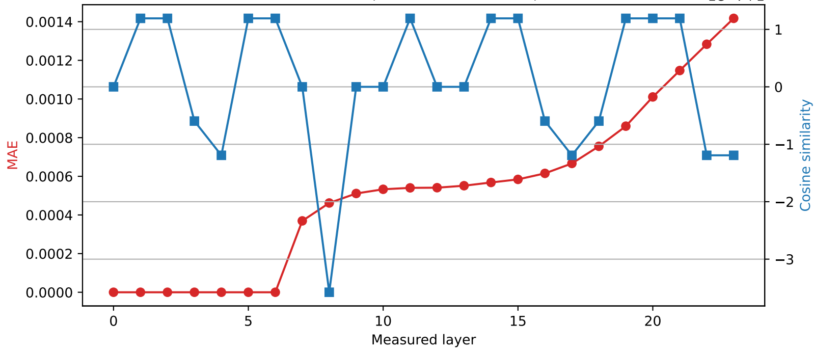
SmolLM2-1.7B-Instruct | Quantized layer 6 | float64 \rightarrow int16
