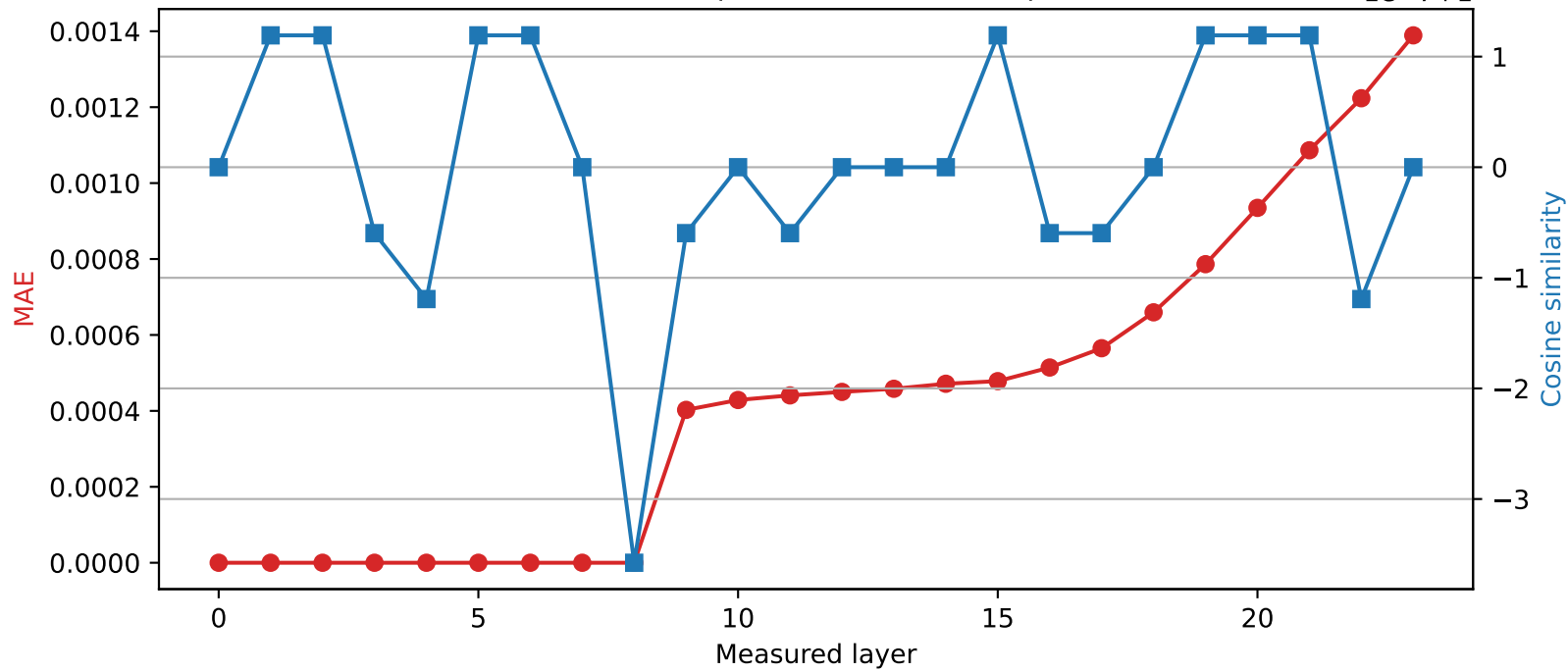
SmolLM2-1.7B-Instruct | Quantized layer 8 | float64 → int16
