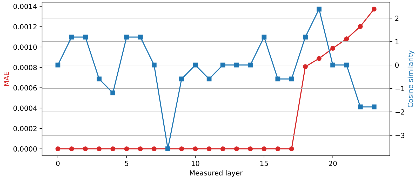
SmolLM2-1.7B-Instruct | Quantized layer 17 | float64 → int16
