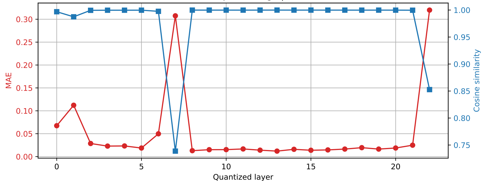
SmolLM2-1.7B-Instruct | Prompt 0 Final RMSNorm output damage | float64 → int8
