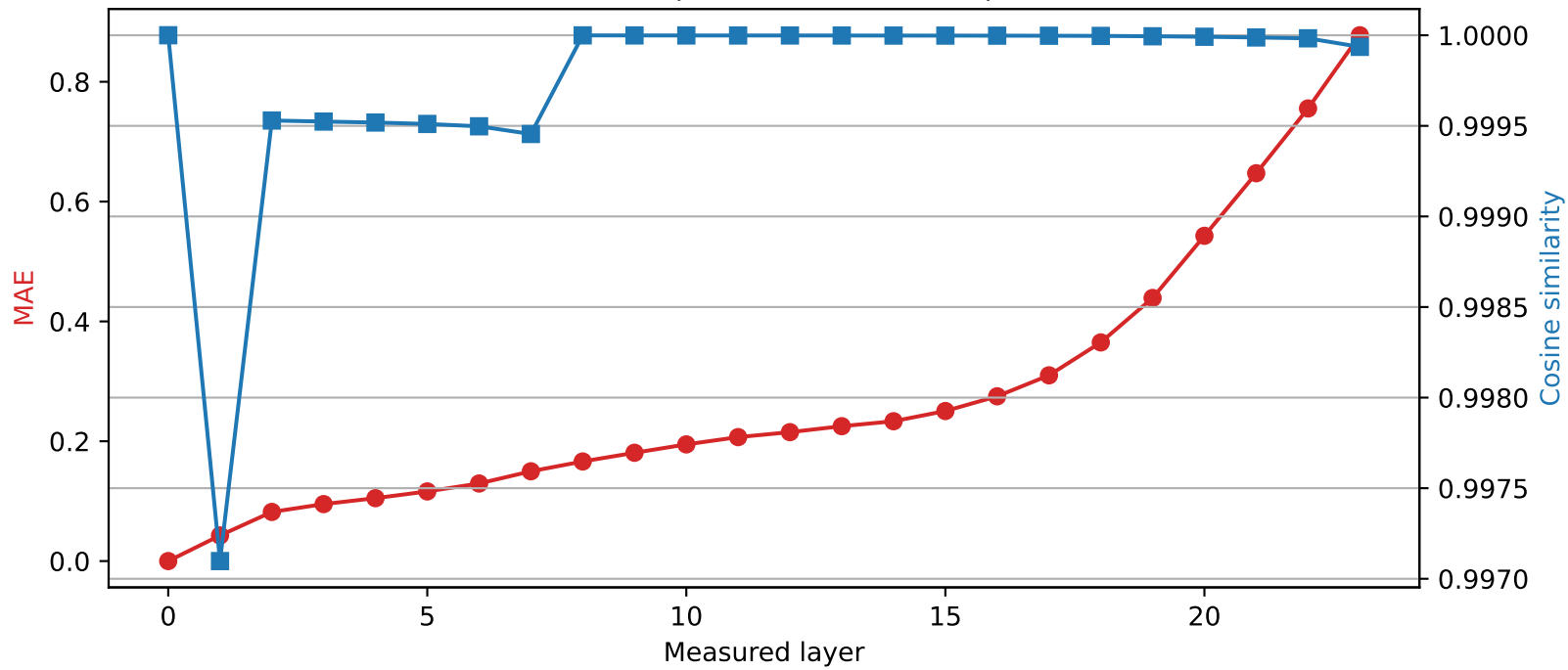
SmolLM2-1.7B-Instruct | Quantized layer 0 | float64 → int8
