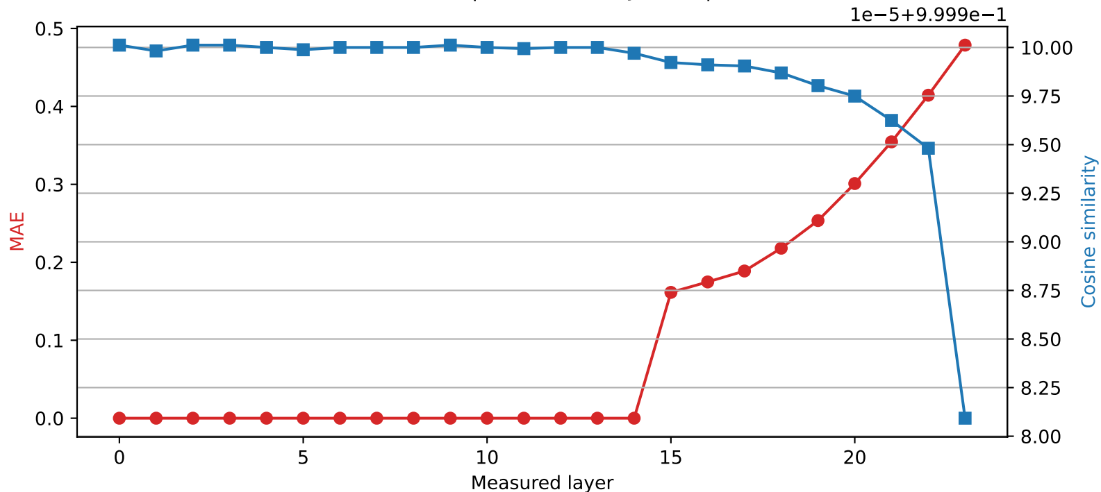
SmolLM2-1.7B-Instruct | Quantized layer 14 | float64 → int8
