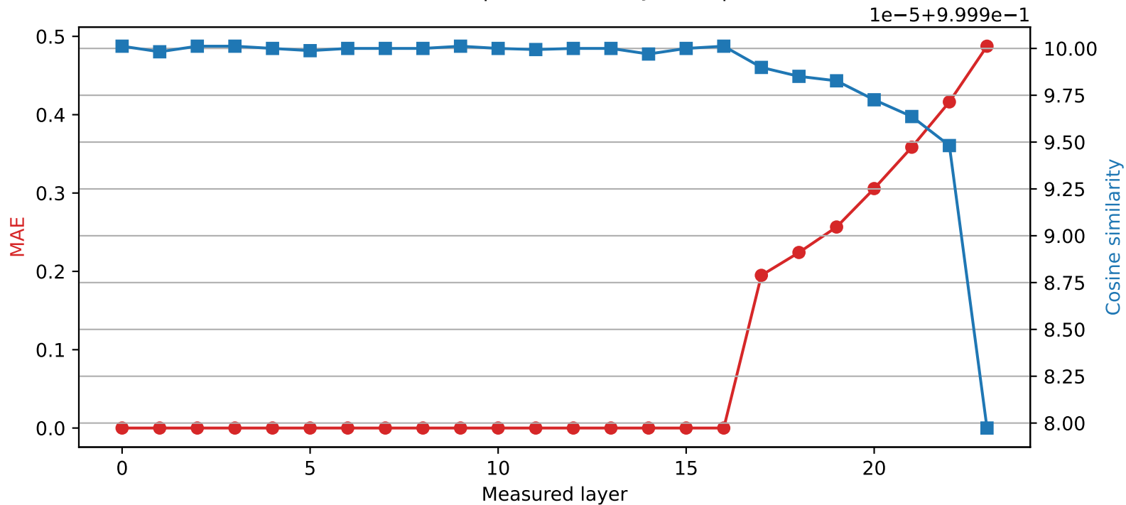
SmolLM2-1.7B-Instruct | Quantized layer 16 | float64 → int8
