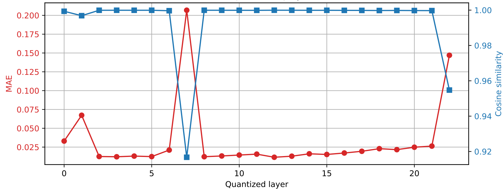
SmolLM2-1.7B-Instruct | Prompt 2 Final RMSNorm output damage | float64 → int8
