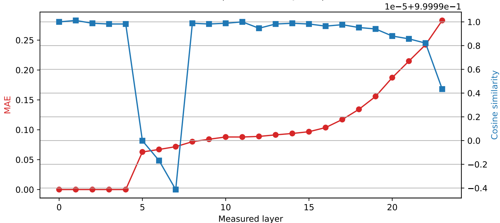
SmolLM2-1.7B-Instruct | Quantized layer 4 | float64 → int8
