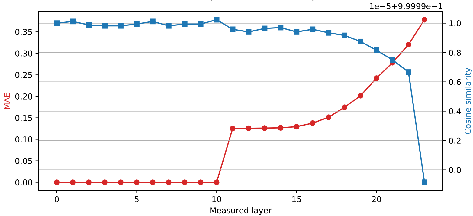
SmolLM2-1.7B-Instruct | Quantized layer 10 | float64 → int8
