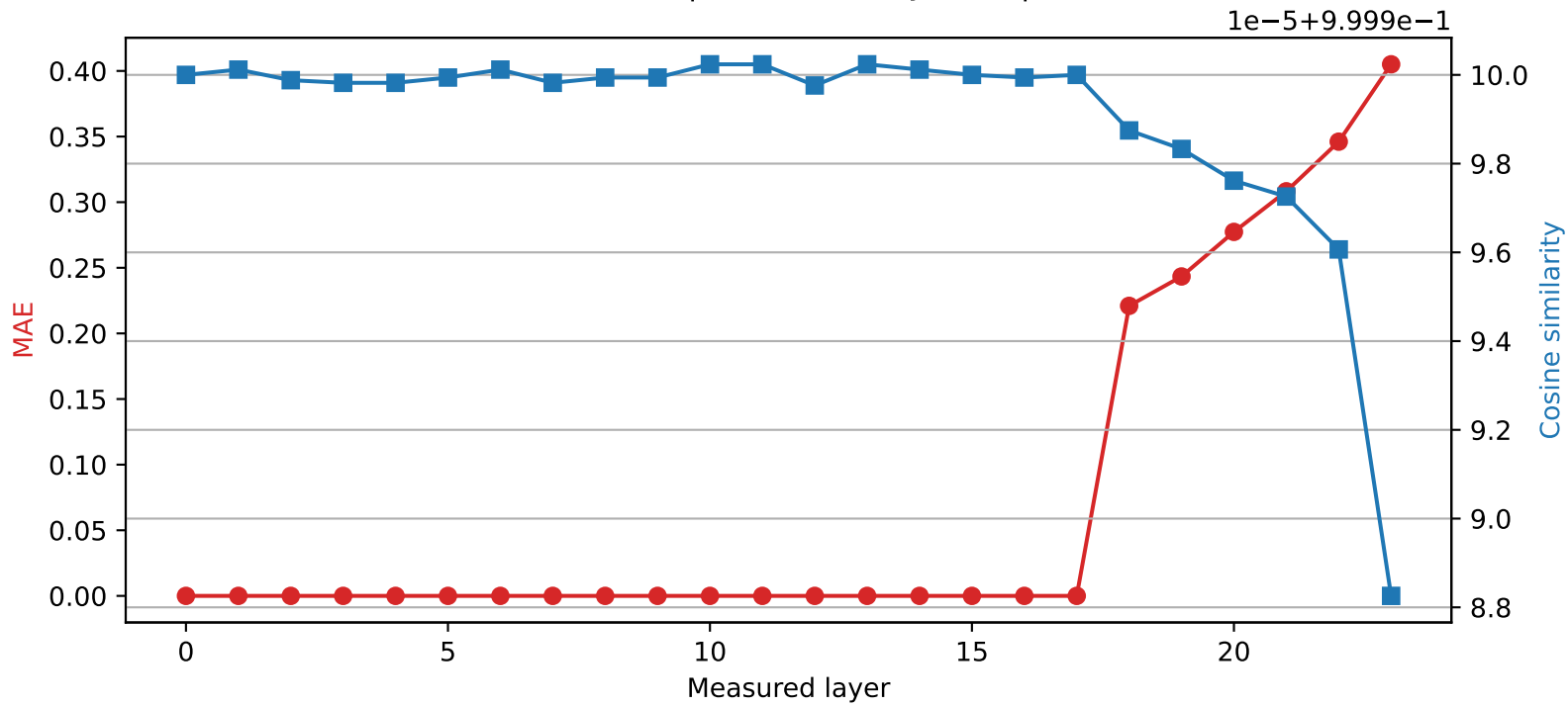
SmolLM2-1.7B-Instruct | Quantized layer 17 | float64 → int8
