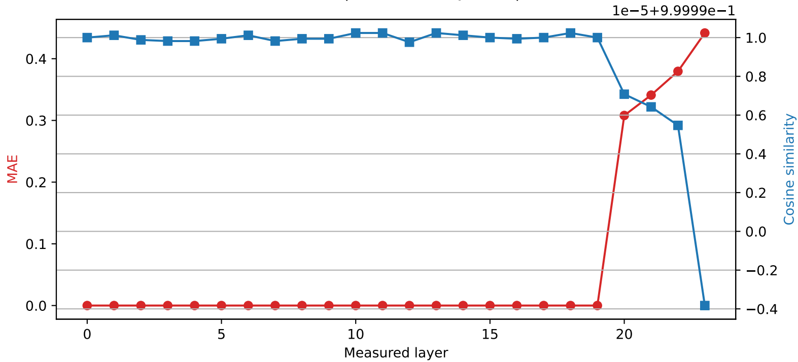
SmolLM2-1.7B-Instruct | Quantized layer 19 | float64 → int8
